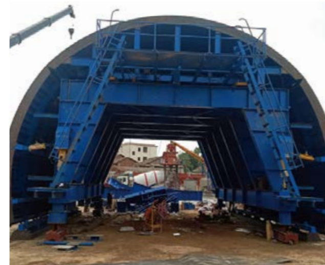
Steel Formwork Tunnel Trolley 钢模体系隧道台车
